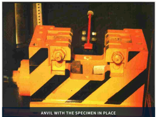
SPECIMEN BEING SET UP FOR THE TEST
