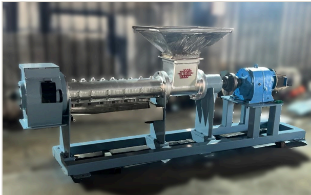
PRE-PRESS MACHINE (EXPELLER) 50-500 TPD
